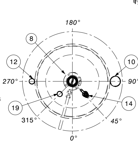
Detail C
